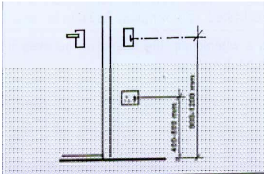
Fig-1. Heights for Switches, Doors, Handrails
