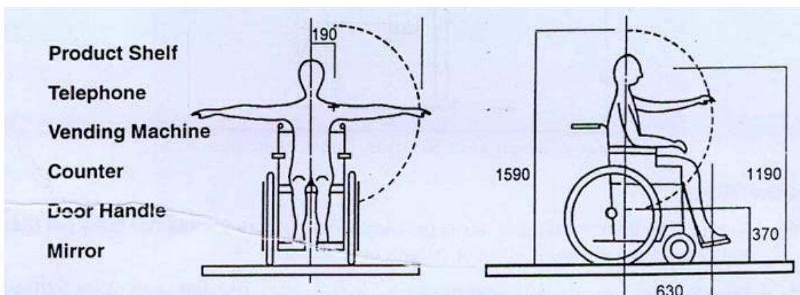
Fig-3. Range of Reach
