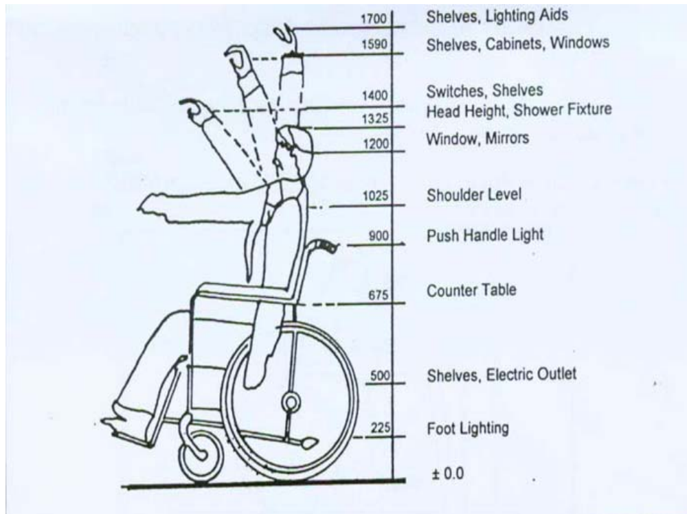
Fig-2. Typical Dimensions for Essential Uses with in easy reach
