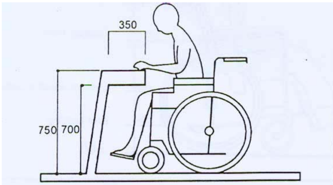
Fig-4. Space required for wheelchair footplate
