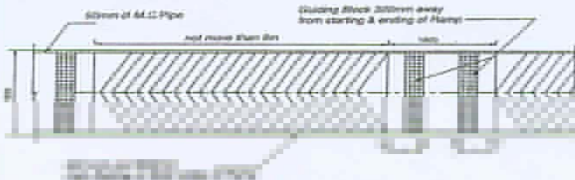
Fig-1. Details of Ramp for Wheelchair users and Disabled persons.
